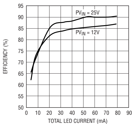
Efficiency (PWM Dimming)
